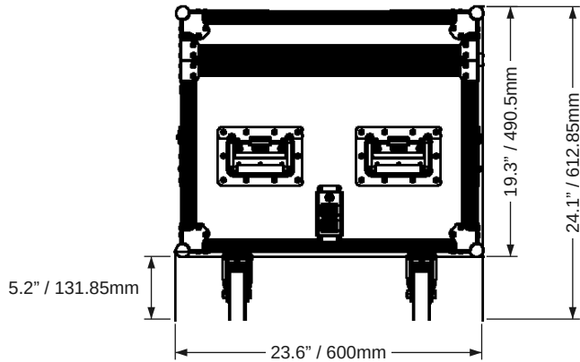
End view, closed (TRUE1 power panel)
