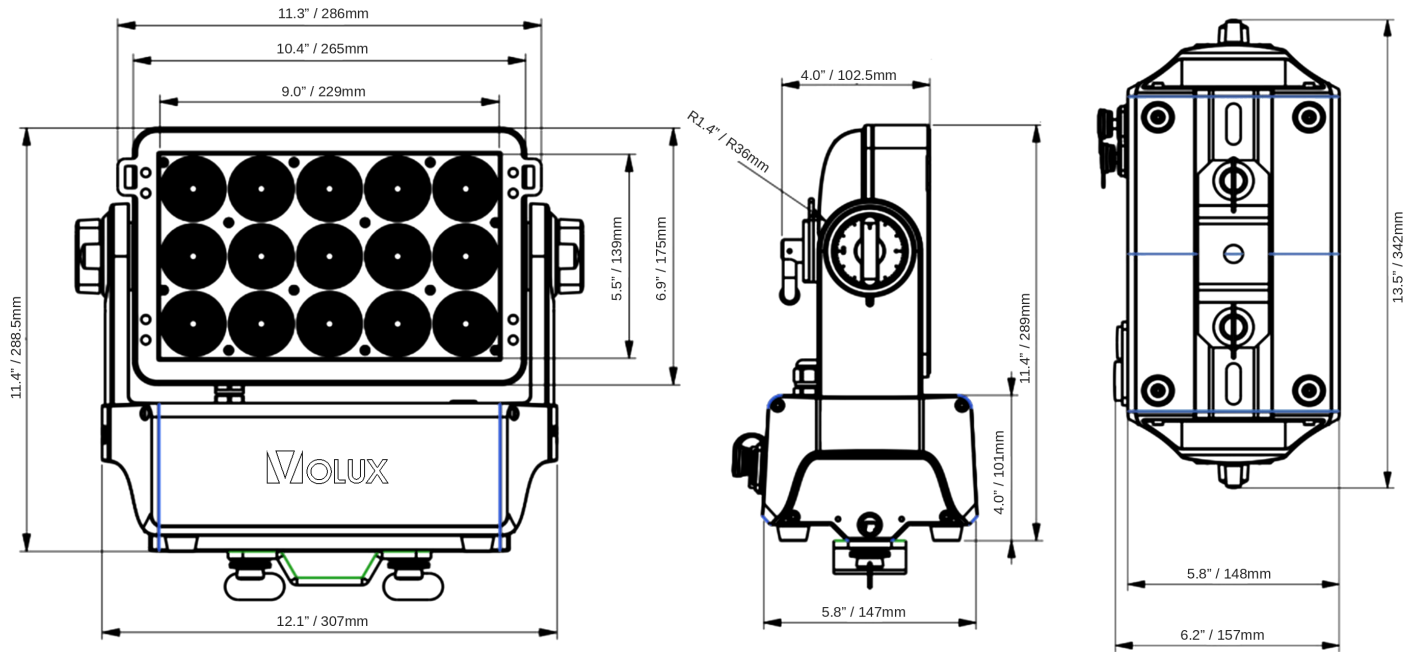
Front (left), side (center) and underside (right) views. Dimensions shown in inches / millimeters.
