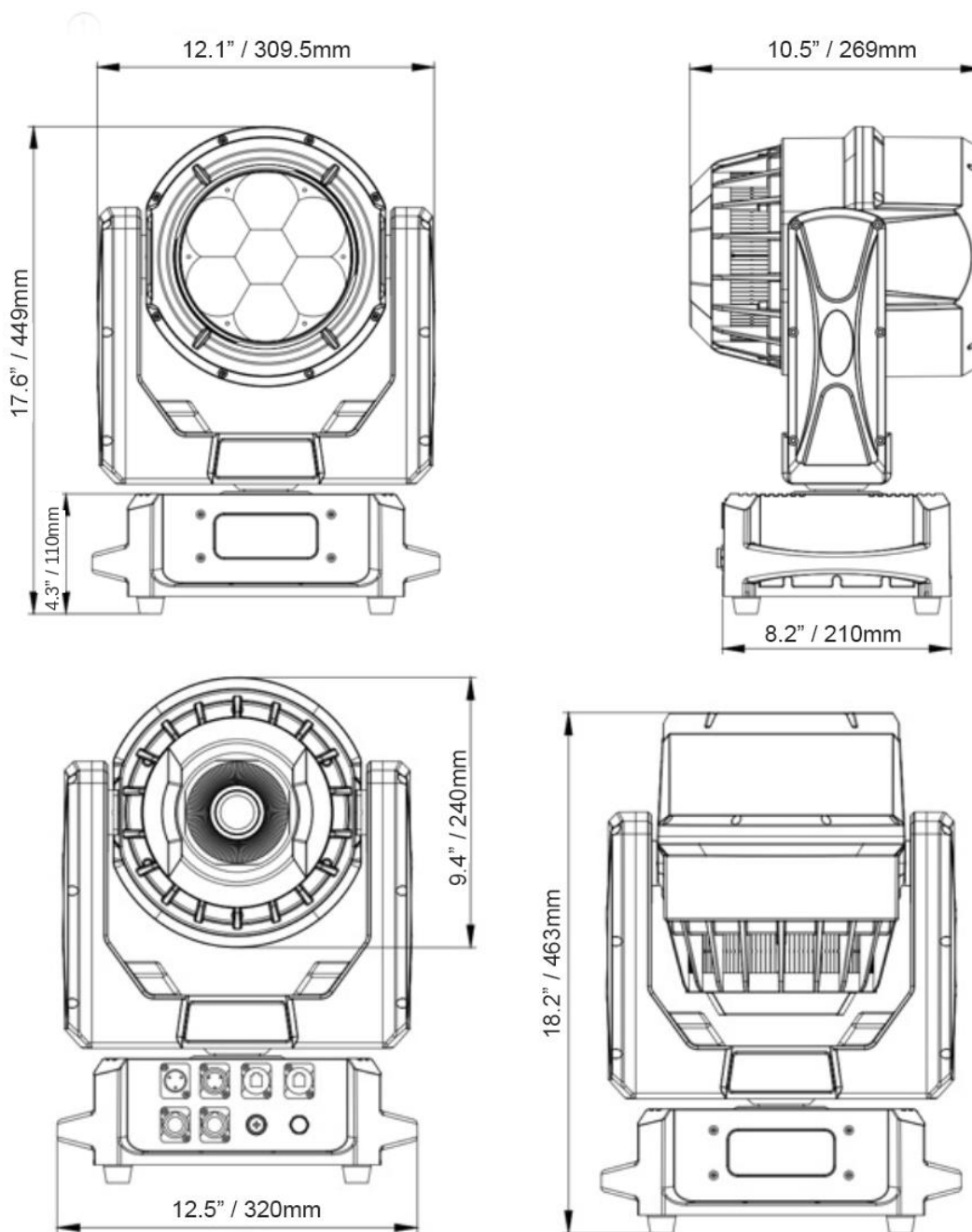
Front and side views (top), rear and side views with head tilted (bottom). Dimensions shown in inches / millimeters.
