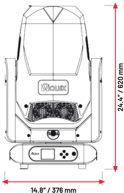
FRONT · HEAD UP
