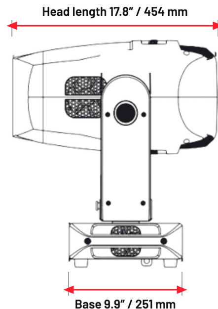
SIDE · HEAD AT 90°
